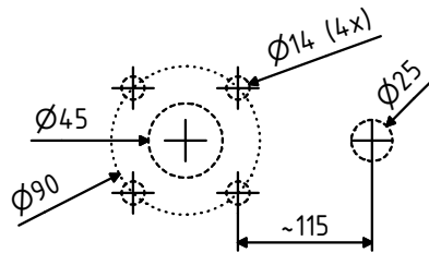
Bench Mounting Holes
